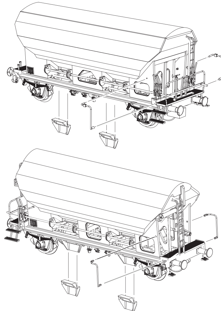
ROCO Oiler 10906
